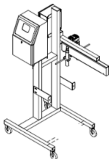
MOBILE MOUNT WITH PRINTER
